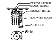
RAIN WATER PERCOLATION DRAWING TYPE -1A
