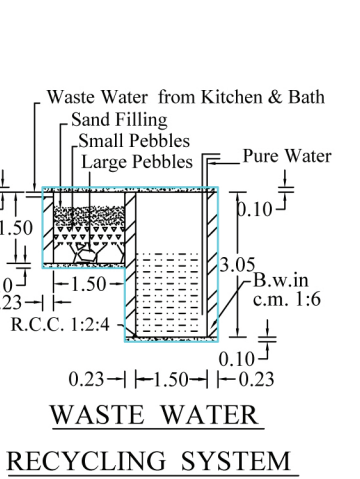
WASTE WATER RECYCLING SYSTEM
