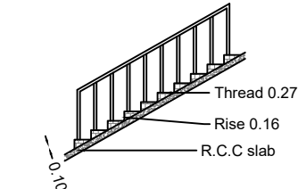
STAIRCASE DETAIL
