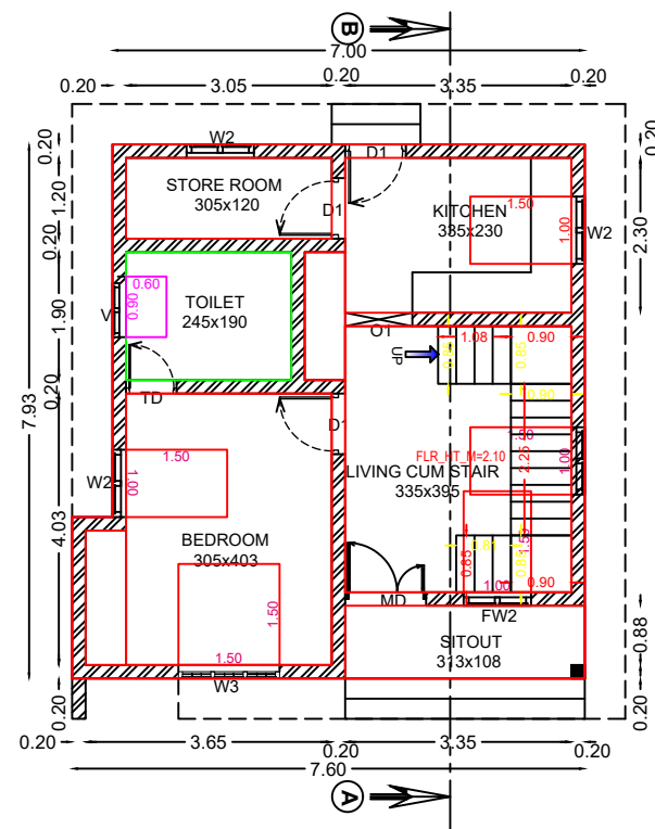
GROUND FLOOR PLAN BUILTUP AREA = 56.98 m 2 (613.10 sq.ft)
