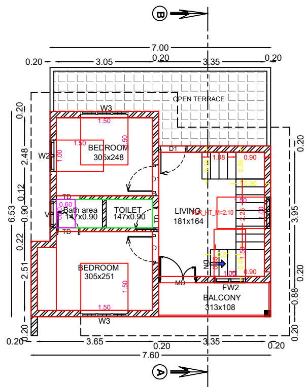
FIRST FLOOR PLAN BUILTUP AREA = 43.26 m 2 (465.47 sq.ft)
