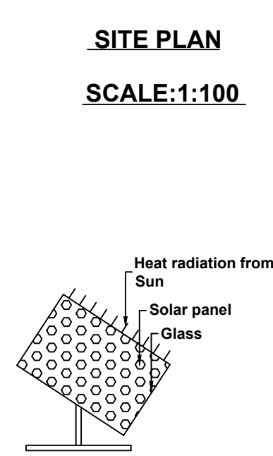
SOLAR SYSTEM
