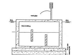
SECTION ON BB
