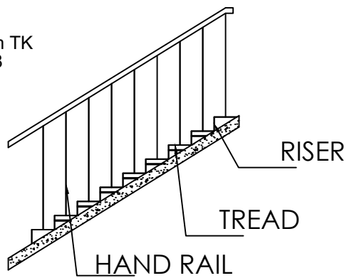
SECTION OF STAIR CASE DETAILS
