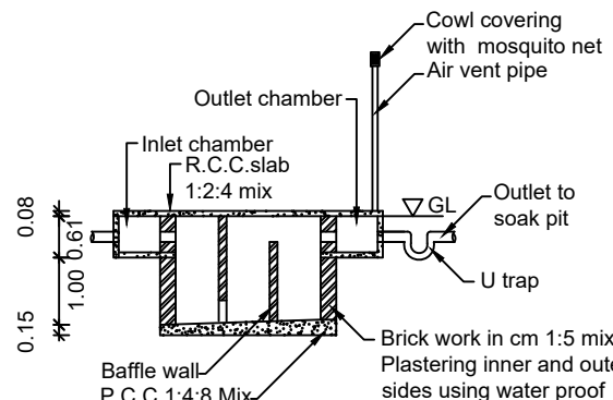
SECTION UV
