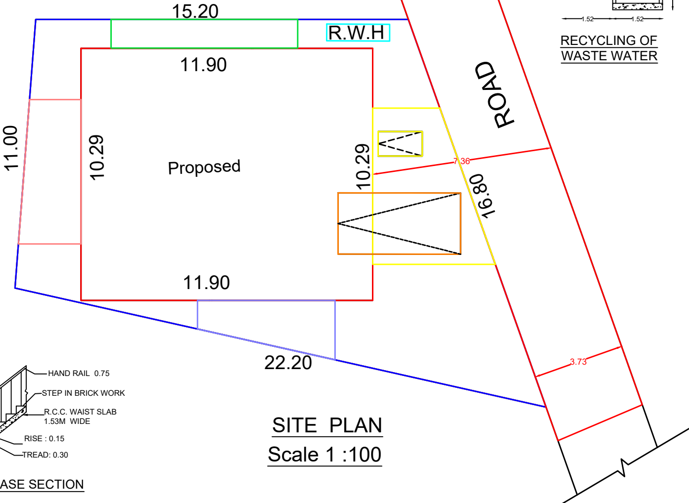
SITE PLAN
