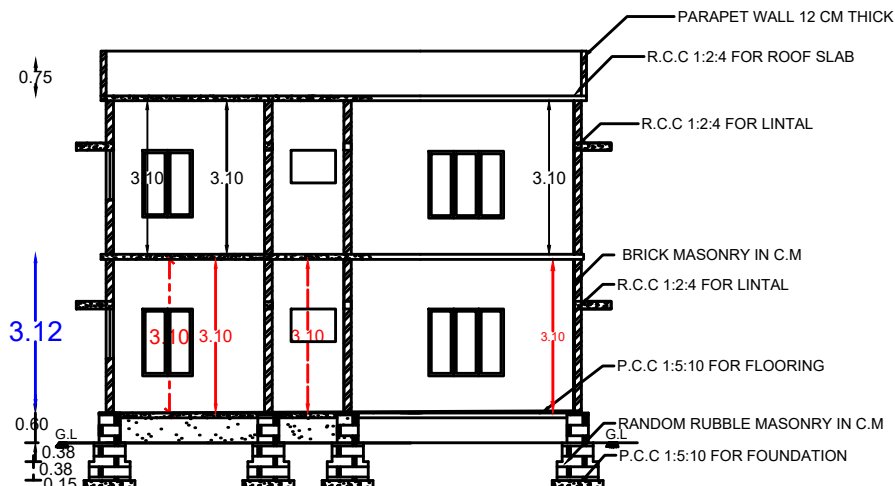
SECTION
