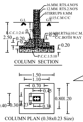
COLUMN SECTION COLUMN PLAN (0.38x0.23 Size)
