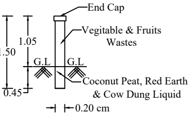
PIPE COMPOSTER
