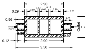
SPECTIC TANK PLAN
