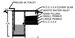
RECYCLING OF WASTE WATER KITCHEN & BATH ROOM
