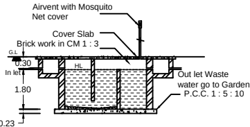
SPECTIC TANK SECTION
