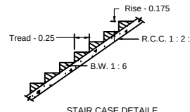
STAIR CASE DETAIL
