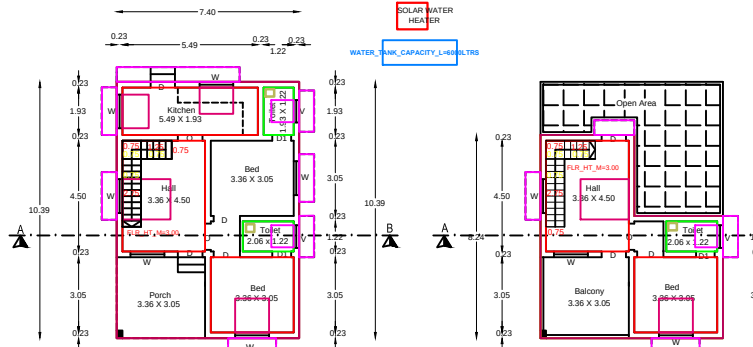
T FLOOR PLAN
