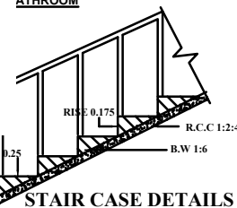
STAIR CASE DETAILS
