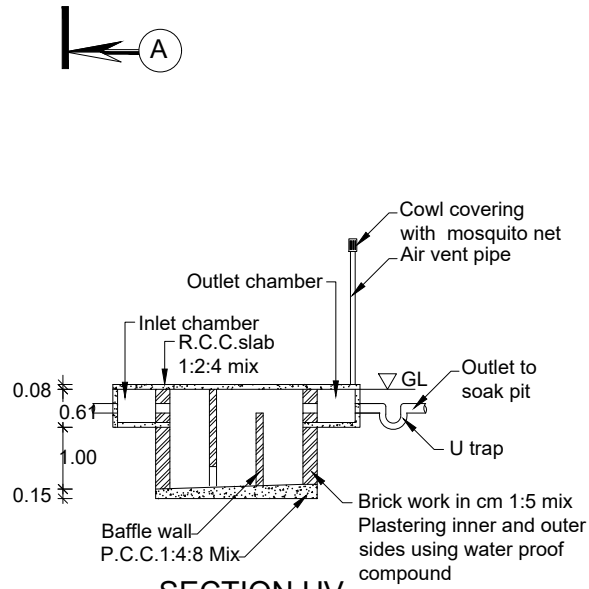
SECTION UV
