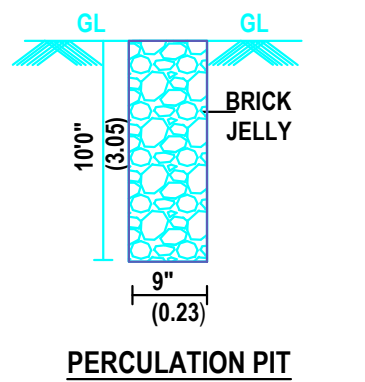
PERCULATION PIT
