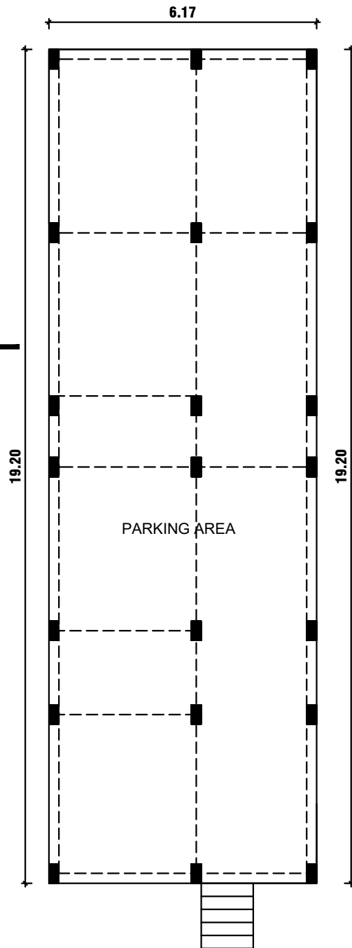
CELLAR FLOOR PLAN(PARKING)
