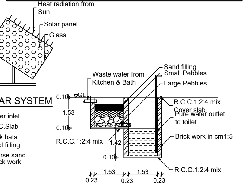
WASTE WATER RECYCLING SYSTEM
