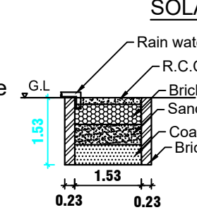
RAIN WATER HARVESTING PIT RWL_CAPACITY_L=5000LTRS
