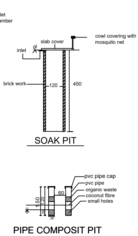
PIPE COMPOSIT PIT
