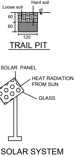
SOLAR SYSTEM
