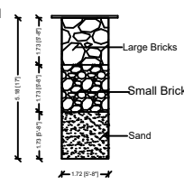
SECTION OF RAIN WATER COLLECTION PITS. (NTS)
