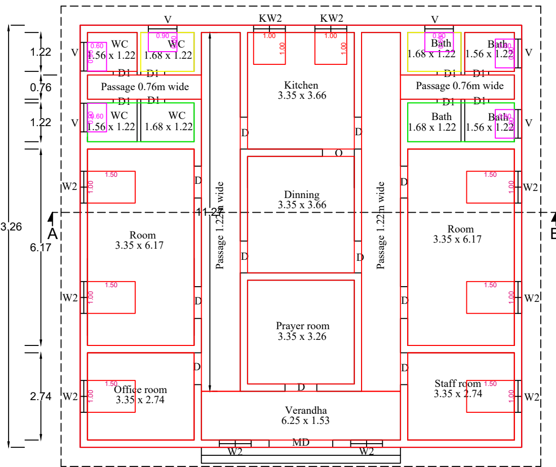
PLAN
