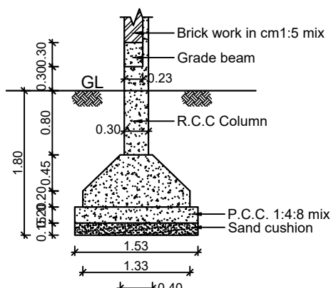
COLUMN DETAILS SCALE 1:50
