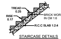
STAIRCASE DETAILS
