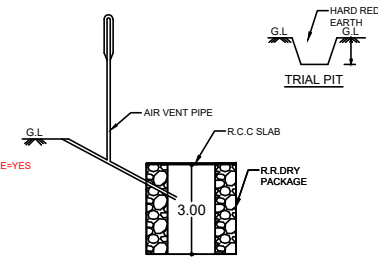
SECTION OF SOAKPIT
