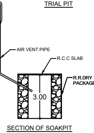
SECTION OF SOAKPIT
