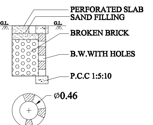
RAIN WATER PERCOLATION DRAWING TYPE -1A
