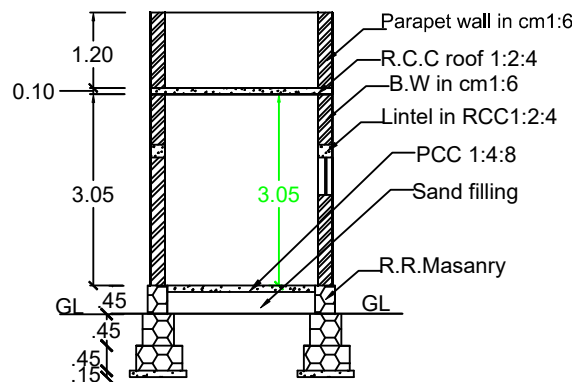
SECTION ON BB
