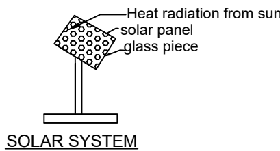
SOLAR SYSTEM
