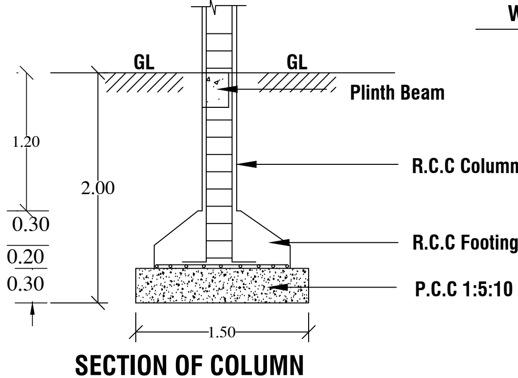
SECTION OF COLUMN
