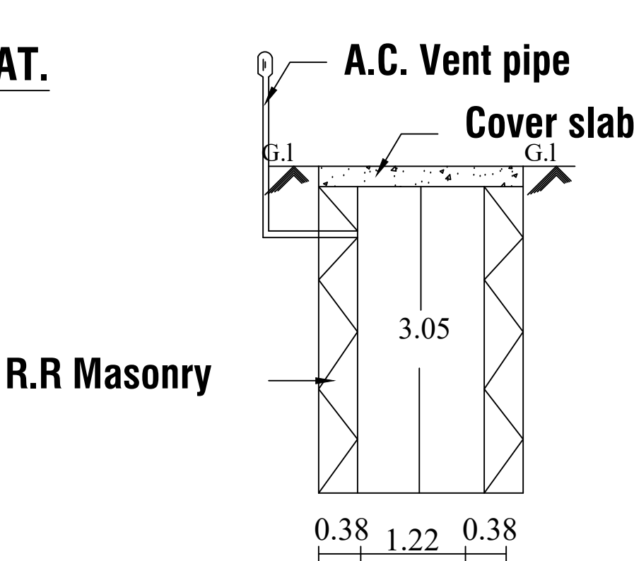
Soakpit section
