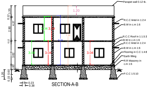
SECTION-A-B
