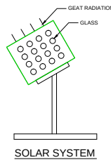
SOLAR SYSTEM
