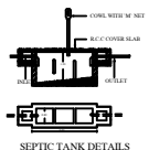
SEPTIC TANK DETAILS
