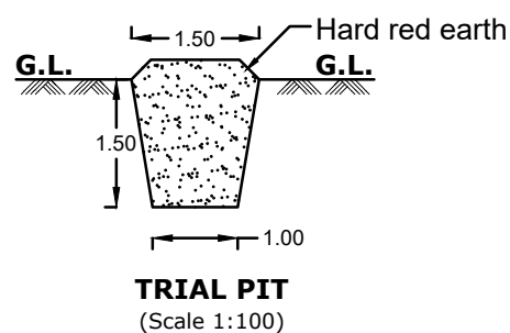
TRIAL PIT (Scale 1:100)
