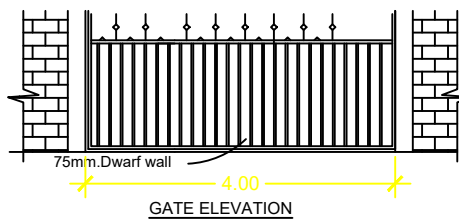
GATE ELEVATION
