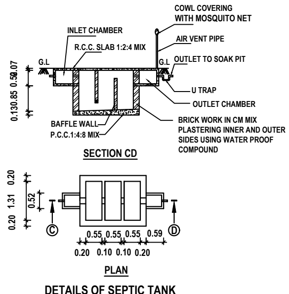
DETAILS OF SEPTIC TANK
