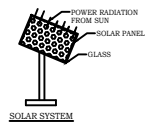
SOLAR SYSTEM
