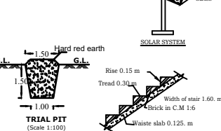
STAIR DETAILS
