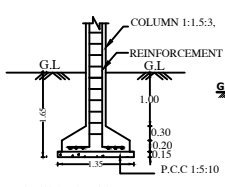
SECTION OF COLUMN
