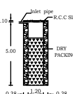
WASTE WATER TANK
