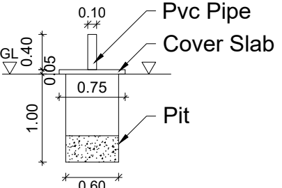
WASTE COMPOST PIT
