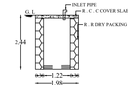
RAIN WATER STORAGE TANK SECTION
