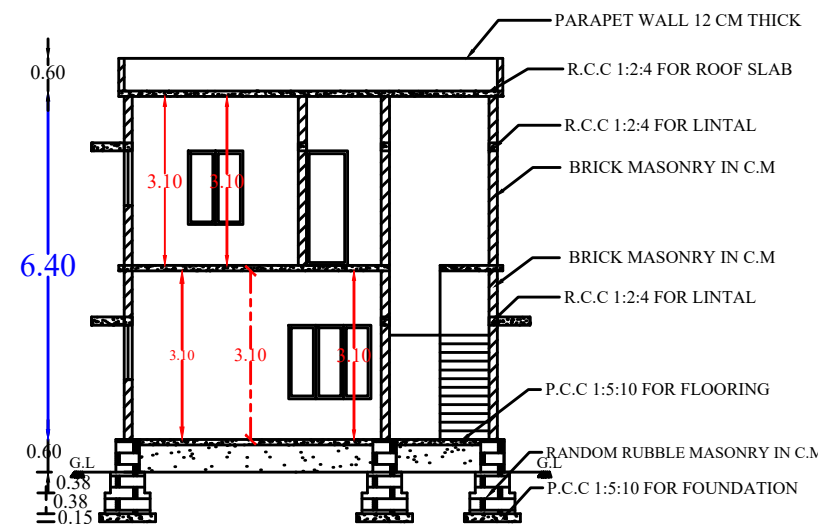
SECTION
