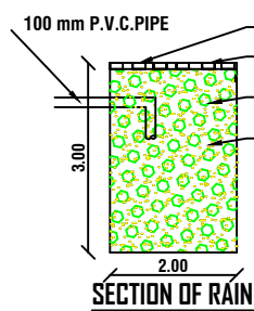
SECTION OF RAIN
