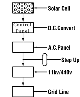
Solar System Flow Diagram
