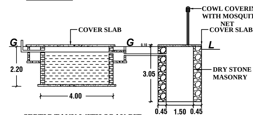
SEPTIC TANK WITH SOAK PIT
