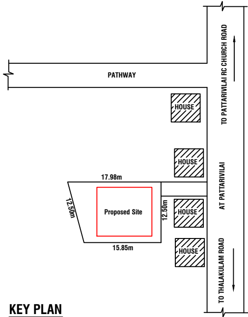
KEY PLAN
