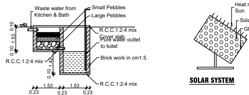
WASTE WATER RECYCLING SYSTEM
