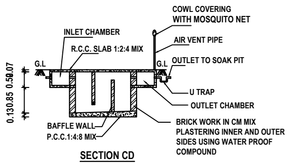
SECTION CD
