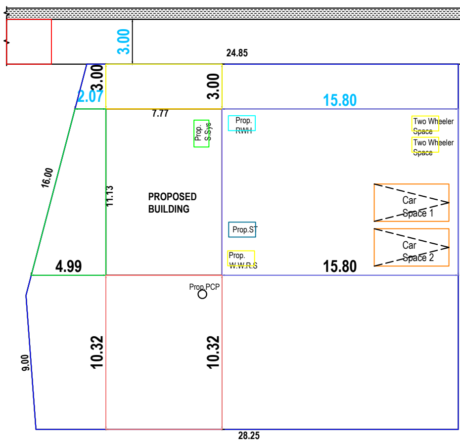
SITE PLAN
