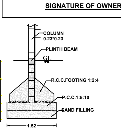
COLUMN DETAILS DETAIL "A"
