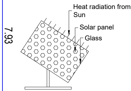
SOLAR SYSTEM
