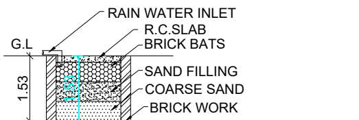
RAIN WATER HARVESTING PIT
