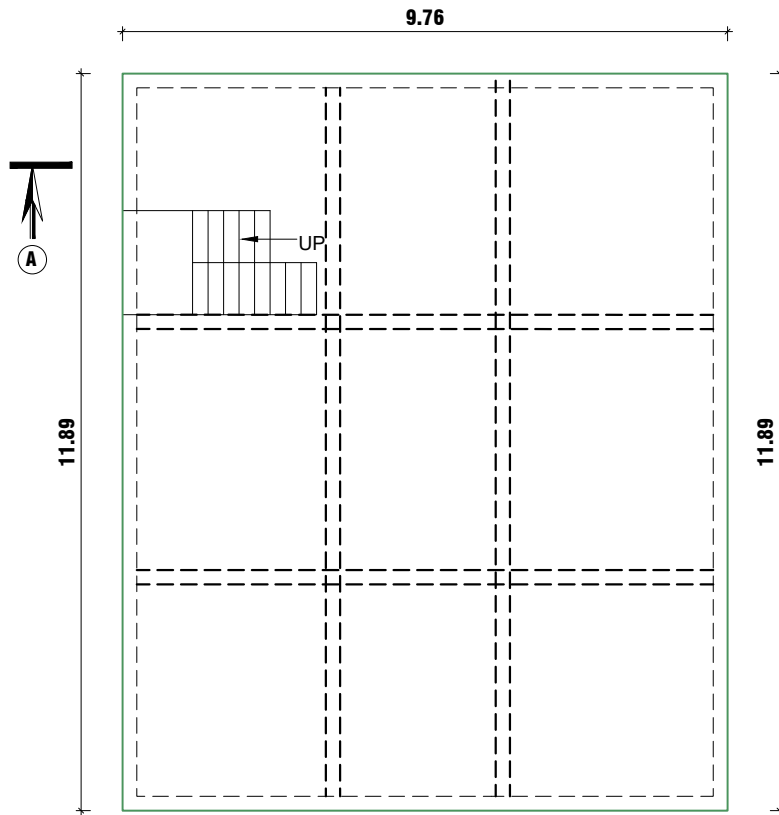
UNDER GROUND FLOOR PLAN
