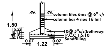
SECTION OF COLUMN
