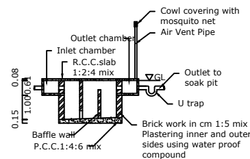
SECTION UV
