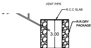
SECTION OF SOAKPIT
