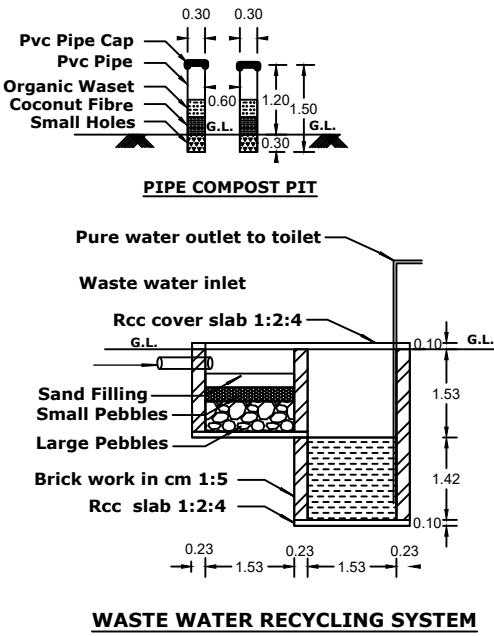
WASTE WATER RECYCLING SYSTEM
