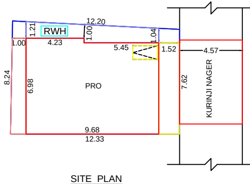
SITE PLAN
