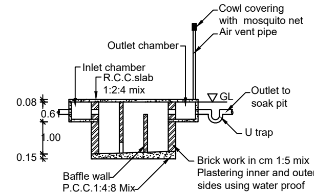
SECTION UV
