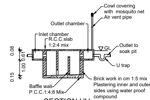
SECTION UV
