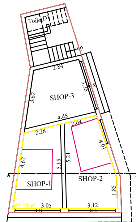
PLAN
