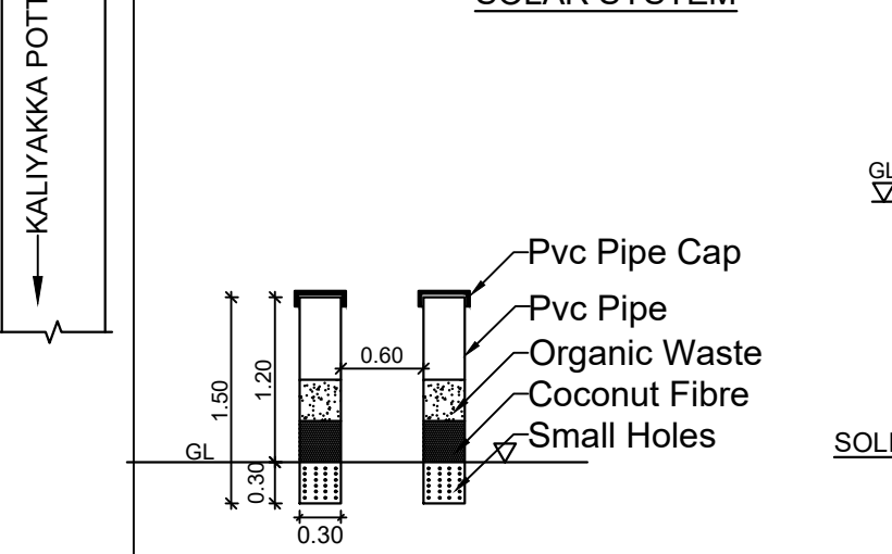
PIPE COMPOST PIT
