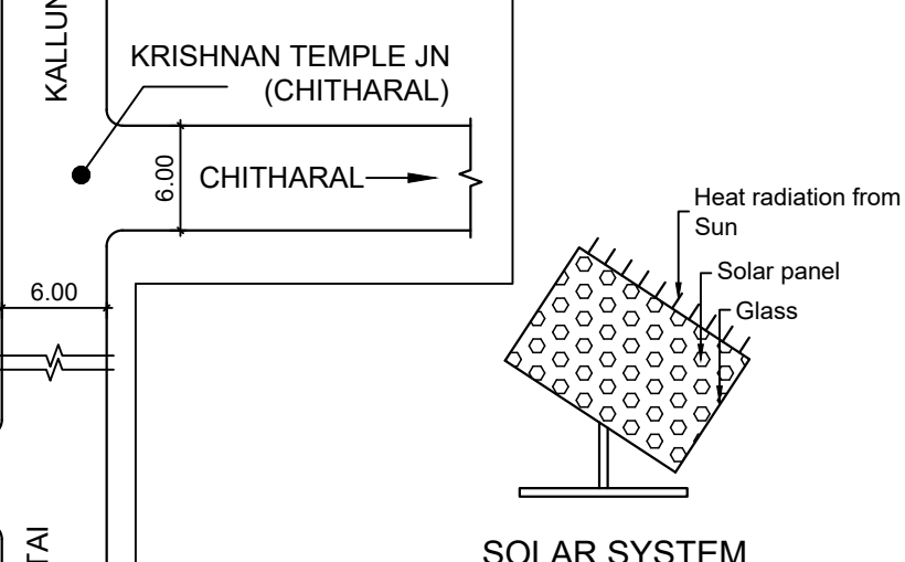
SOLAR SYSTEM
