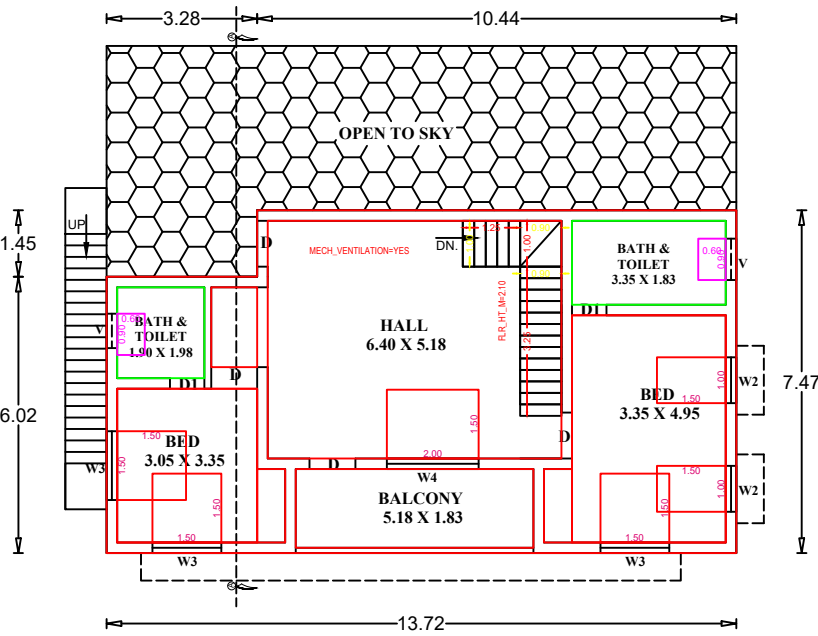
PLAN (FIRST FLOOR)
