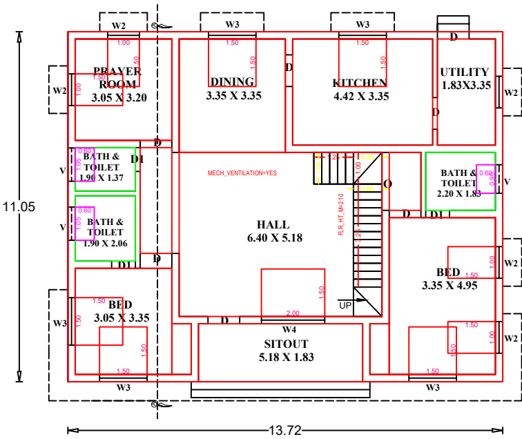
PLAN (GROUND FLOOR)
