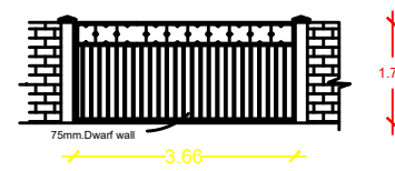
GATE ELEVATION
