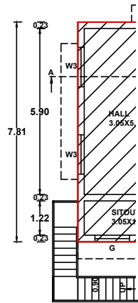
EXISTING GROUND FLOOR PLAN
