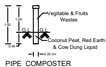
PIPE COMPOSTER
