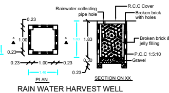
RAIN WATER HARVEST WELL RWH_CAPACITY_L=6642LTRS
