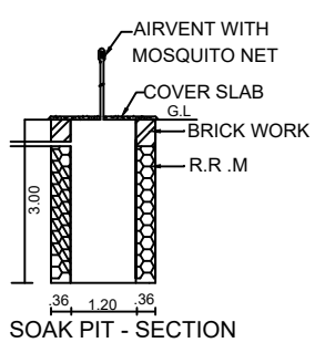
SOAK PIT - SECTION
