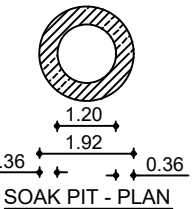
SOAK PIT - PLAN
